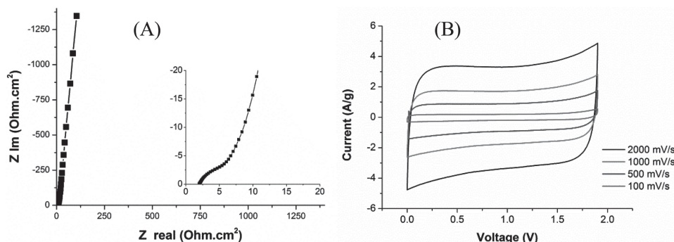
Figure 3. MWNT/graphene yarn tested in a two electrode configuration. (a) Nyquist plot, (b) CV at varying scan rates. Electrolyte is 1 M LiClO 4 /acetonitrile. Mass of each yarn is 0.15 mg with a 50 μm diameter and 5 cm length.
