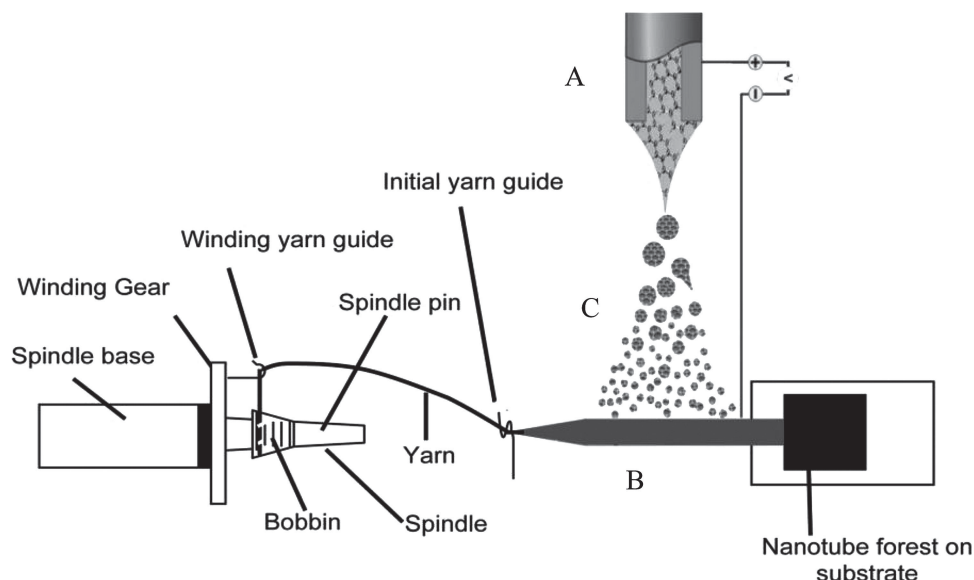
Figure 1. Schematic diagram of continuously produced hybrid CNT/graphene yarn. (A) Electrospinning setup used for graphene deposition; (B) MWNT sheet drawn from spinable forest and employed as graphene collector; (C) graphene dispersion (electrospray).
